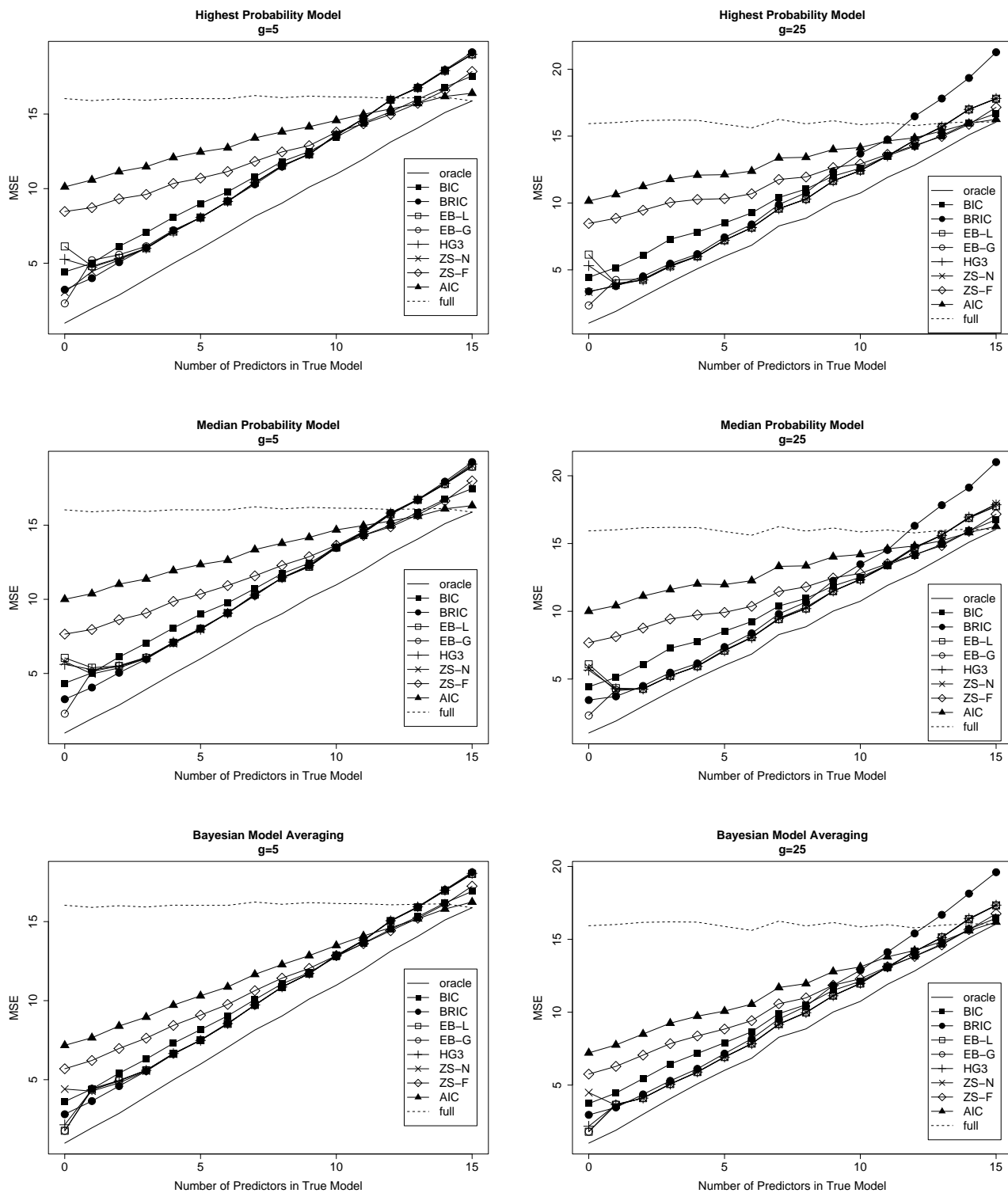
Figure 1: Average MSE from 1000 simulations for each method with p = 15 and n = 100 using the oracle (—), AIC (▲), BIC (■), BRIC (●), EB-local (□), EB-global (○), hyper- g with a = 3 (+), Zellner-Siow null (×), Zellner-Siow full (◇), and full model (- -).
