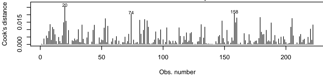
Cook's distance plot
