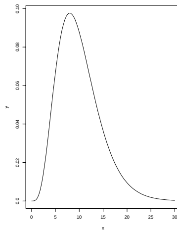
Figure 4.1: Density of \chi^2 distribution with 10 degrees of freedom
