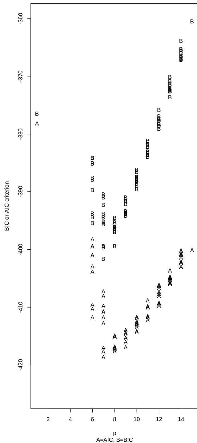
BIC,AIC vs. p
