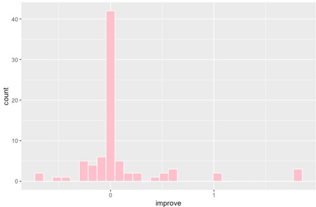
Distribution of improved score
